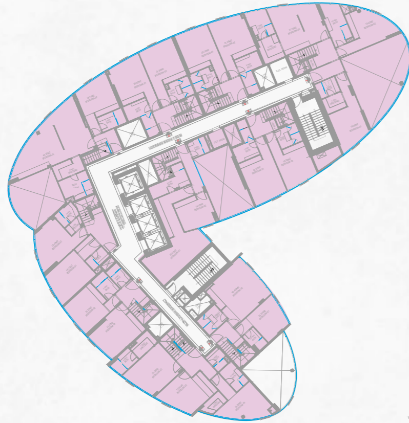
Tower A Duplex - 15th Floor (First Floor)
