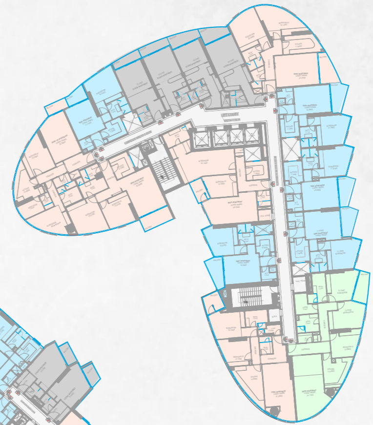
Tower C2 2nd - 19th Floor
