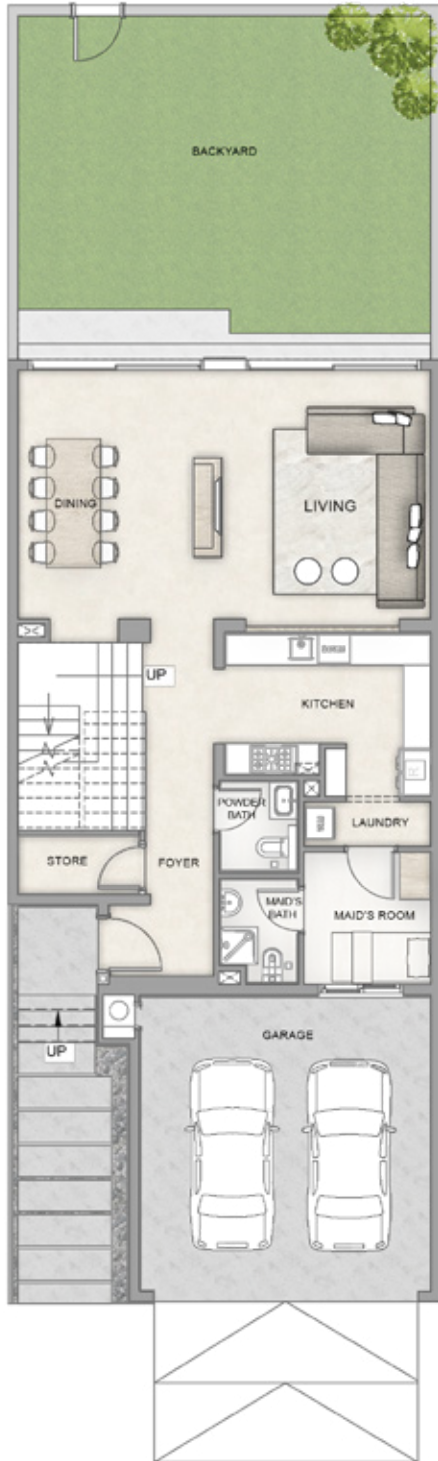
Ground Floor
